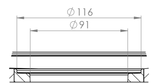
DETAIL C SCALE 1:2
